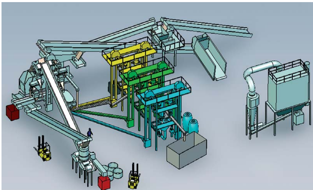
KAHL Recycling plant for waste tyres
